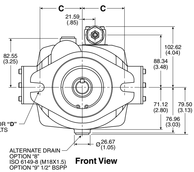
SHAFT OPTION "K" (ø 25mm REF) 8mm x 7mm KEY MAX TORQUE = 336.4 N·m (2,990 IN-LBS)
